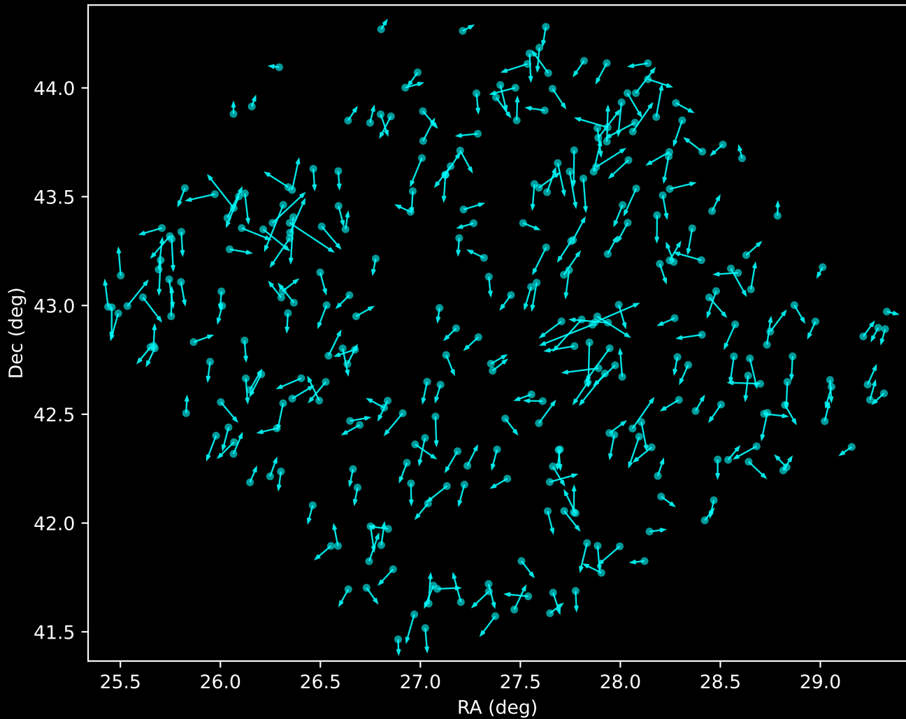
APOGEE DR17 Noise Stream Proper Motion Vectors (n=309)
