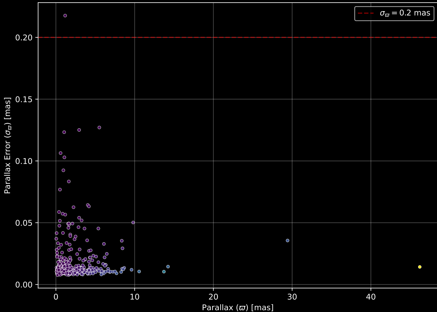
APOGEE DR17 Field: [K12_074+15] Parallax Quality (n= 573)
