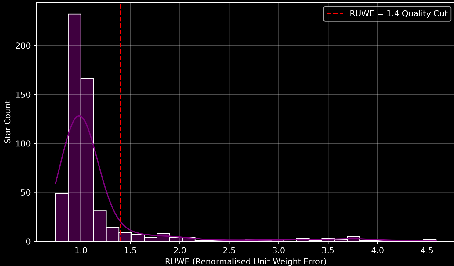
GAPOGEE DR17 Field [K12_074+15] RUWE Distribution (n= 557)
