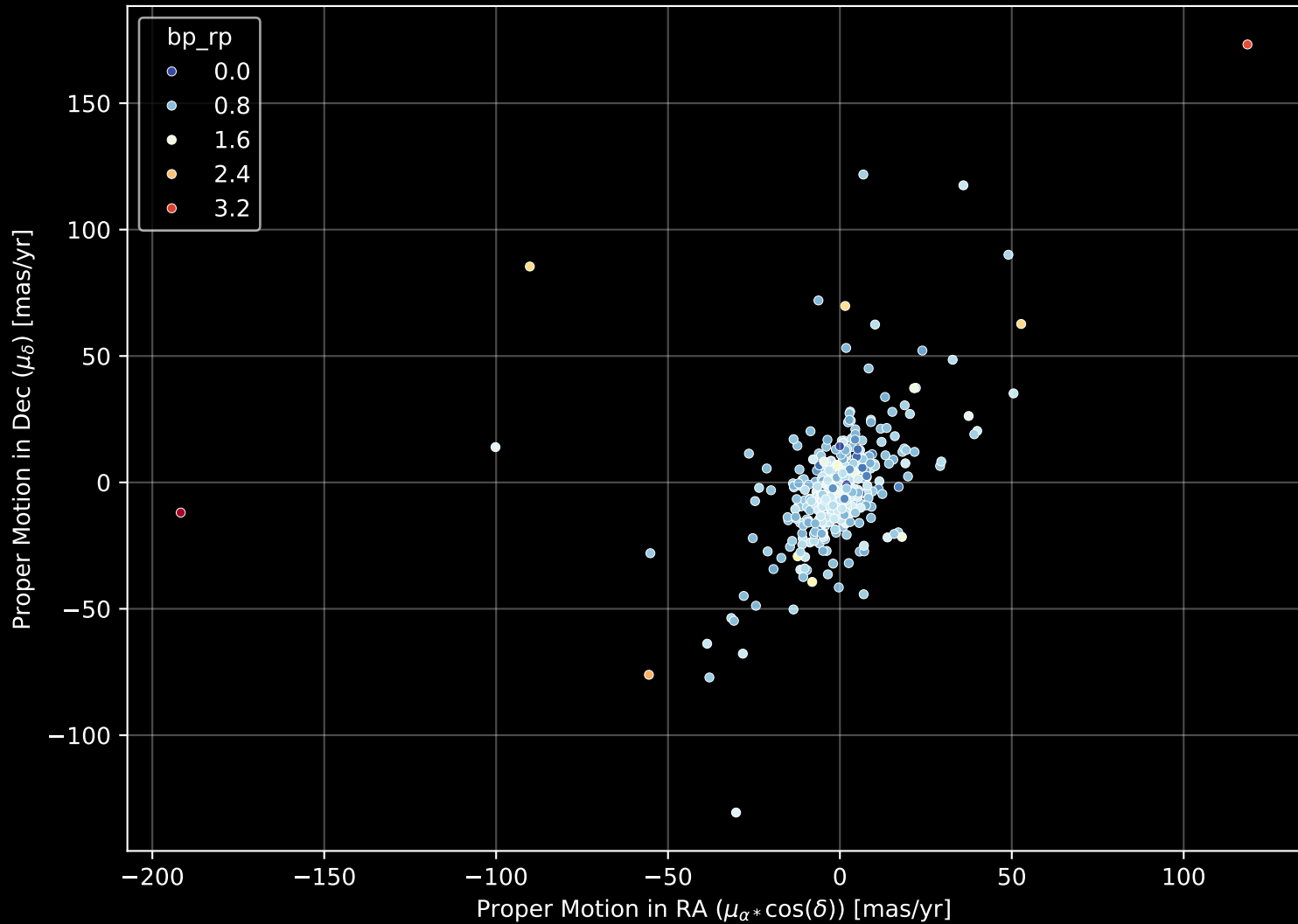
APOGEE DR17 Field: [K12_074+15] Proper Motion Diagram (n= 573)
