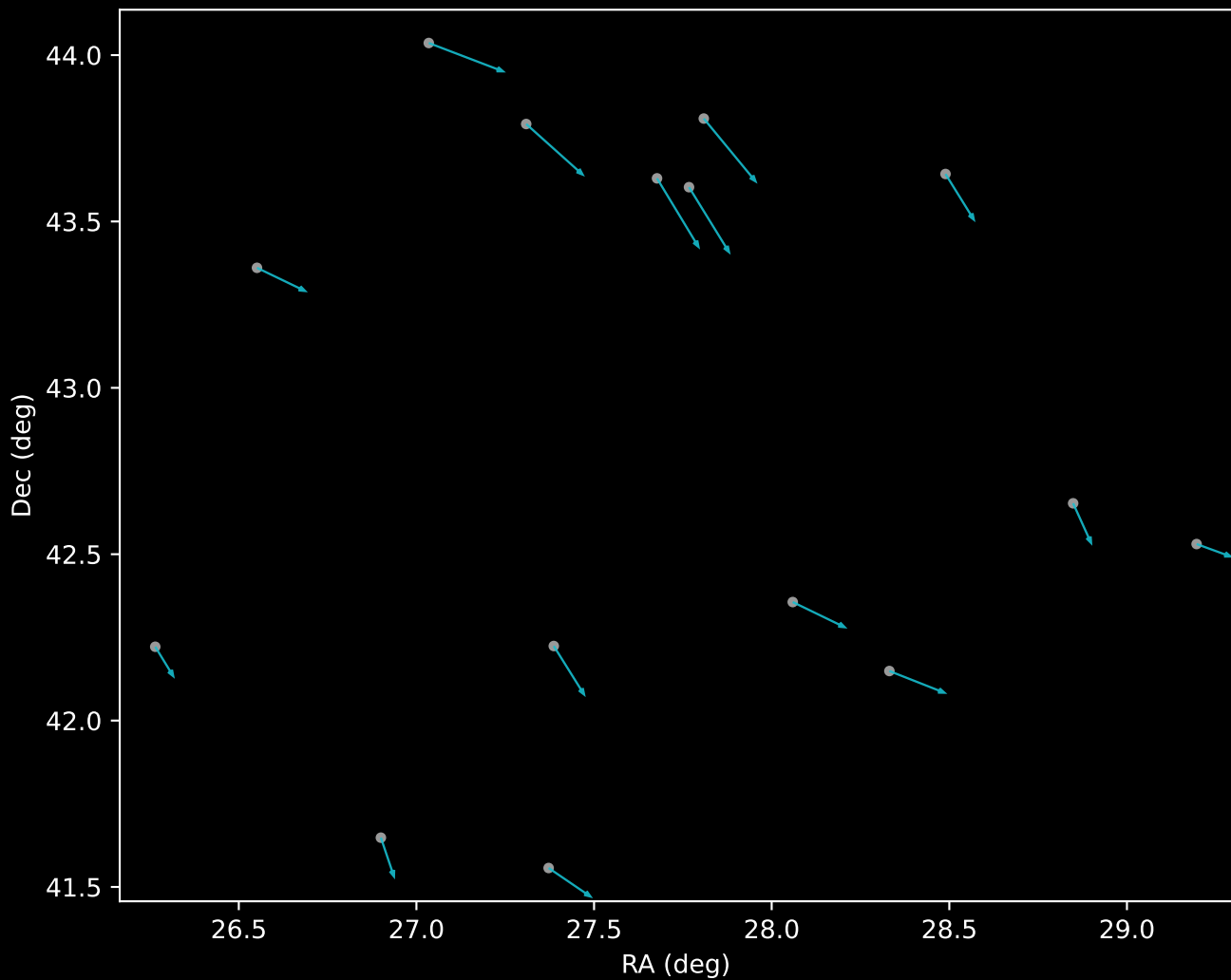
APOGEE DR17 Cluster 18 Proper Motion Vectors (n=15)
