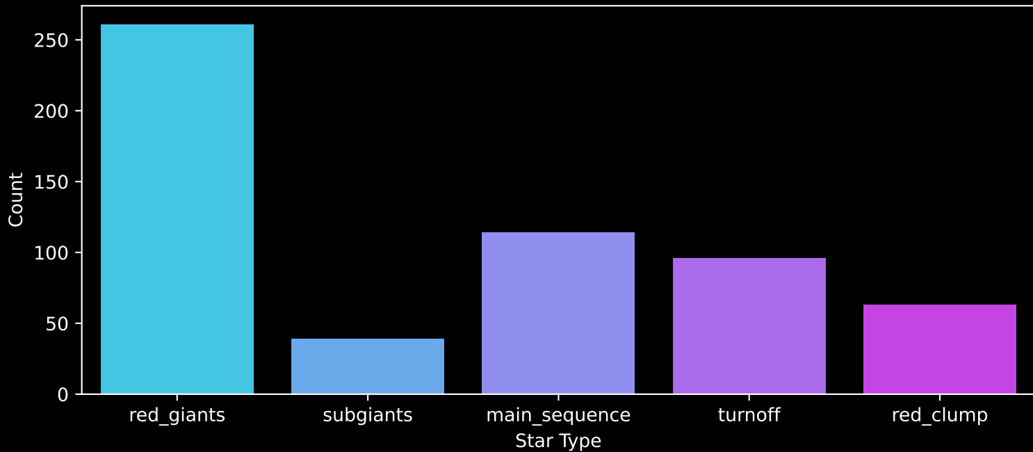
APOGEE DR17 Field: [K12_074+15] Count plot of Star Type
