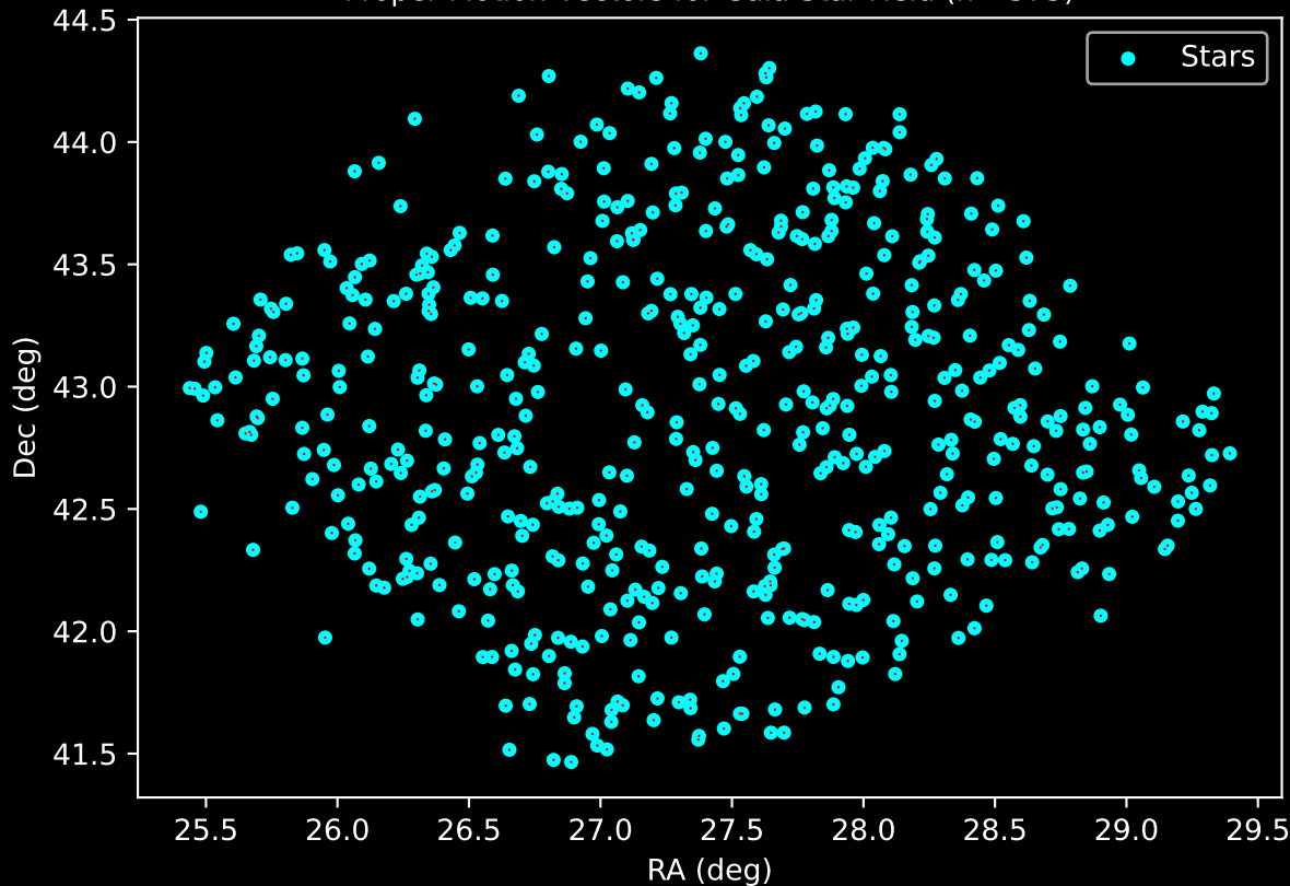
APOGEE DR17 Field: [K12_074+15] Proper Motion Vectors for Gaia Star Field (n= 573)
