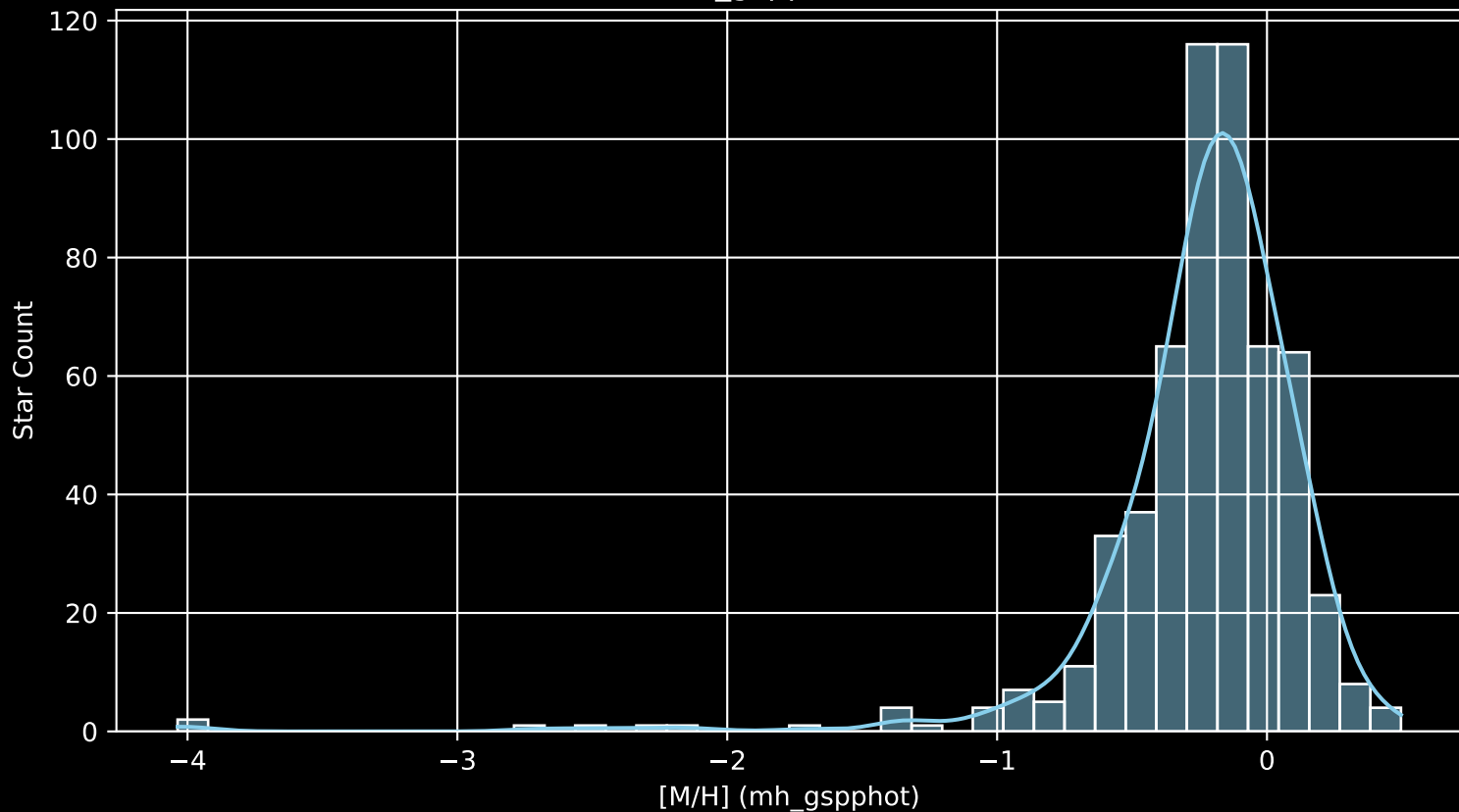
APOGEE DR17 Field: [K12_074+15] [M/H] (mh_gspphot) (n= 570)
